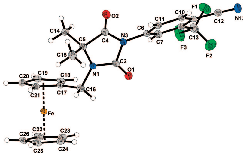
Figure 1. X-ray crystal structure of 1 . Selected bond lengths (Å) and angles (deg): Fe–Cent(1) 1.649(2); Fe–Cent(2) 1.644(1); C 17 –C 16 1.497(2); C 16 –N 1 1.4671(18); N 1 –C 2 1.3467(18); C 2 –N 3 1.4286(18); N 3 –C 4 1.3875(18); C 4 –C 5 1.5313(19); C 5 –N 1 1.4696(18); N 3 –C 6 1.4194(18); C 9 –C 12 , 1.446(2); C 12 –N 12 1.144(2); C 8 –C 13 , 1.501(2); C 2 –O 1 , 1.2120(18); C 4 –O 2 , 1.2045(18); C 21 –C 17 –C 18 , 107.63(13); C 17 –C 16 –N 1 112.66(12); N 1 –C 2 –N 3 , 107.04(12); C 2 –N 3 –C 4 110.87(11); N 3 –C 4 –C 5 107.23(12); C 4 –C 5 –N 1 101.14(11); C 5 –N 1 –C 2 113.50(11).
