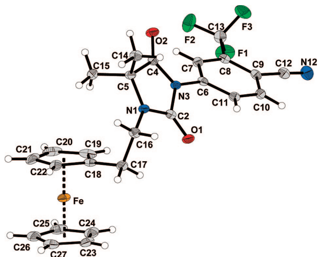
Figure 2. X-ray crystal structure of 2 . Selected bond lengths (Å) and angles (deg): Fe–Cent(1), 1.646(1); Fe–Cent(2), 1.645(1); C 18 –C 17 1.492(3); C 17 –C 16 1.528(3); C 16 –N 1 1.468(2); N 1 –C 2 1.334(2); C 2 –N 3 1.431(2); N 3 –C 4 1.388(2); C 4 –C 5 1.528(2); C 5 –N 1 1.468(2); N 3 –C 6 1.417(2); C 9 –C 12 , 1.444(2); C 12 –N 12 1.143(2); C 8 –C 13 , 1.503(2); C 2 –O 1 , 1.211(2); C 4 –O 2 , 1.206(2); C 19 –C 18 –C 22 , 106.83(17); C 18 –C 17 –C 16 112.66(15); C 17 –C 16 –N 1 113.32(15); N 1 –C 2 –N 3 , 107.29(14); C 2 –N 3 –C 4 110.45(14); N 3 –C 4 –C 5 107.23(14); C 4 –C 5 –N 1 101.21(13); C 5 –N 1 –C 2 113.57(14).
